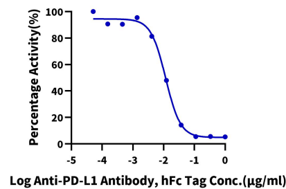
Inhibition of Human PD-L1 and Biotinylated Human PD-1 Binding 0.1µg Human PD-L1, His Tag Per Well
